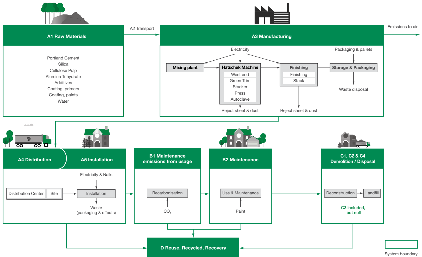
FIGURE 2 SYSTEM BOUNDARY
