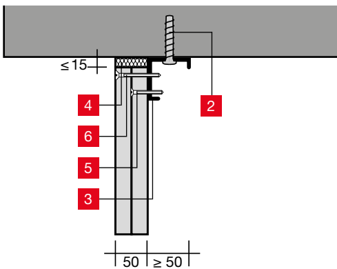
Detail H
