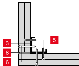
Detail G
