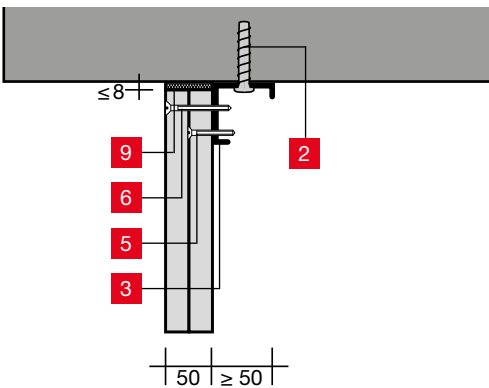
Detail H
