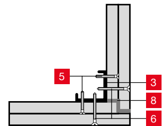
Detail I
