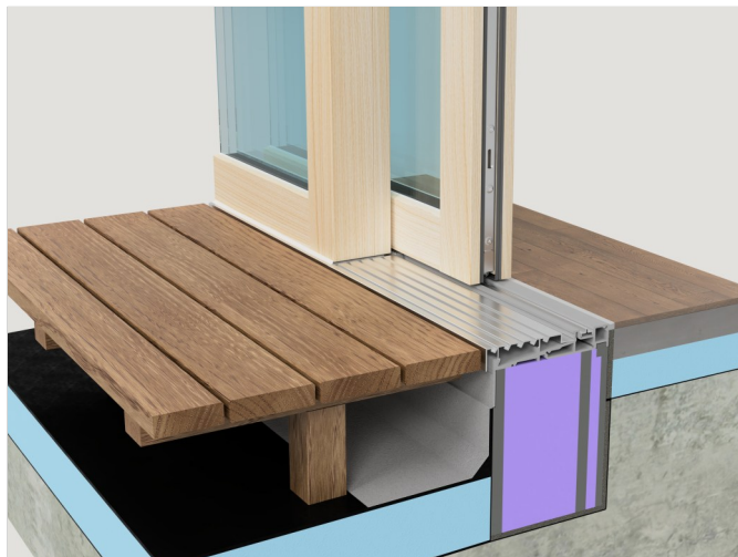
duraslide wood
