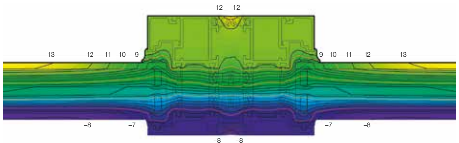
Isothermendiagramm durafold comfort+, Mittelpartie
