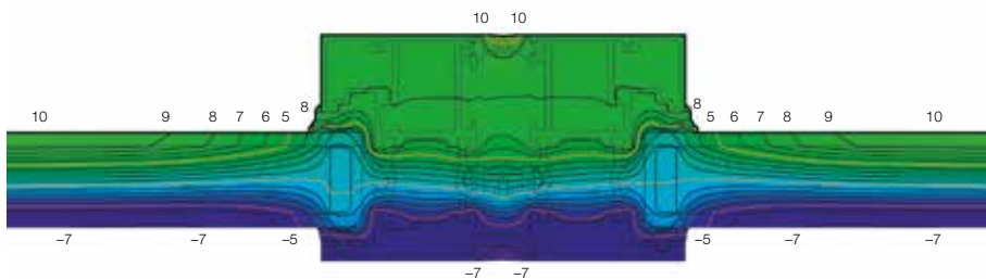
Isothermendiagramm durafold comfort, Mittelpartie
