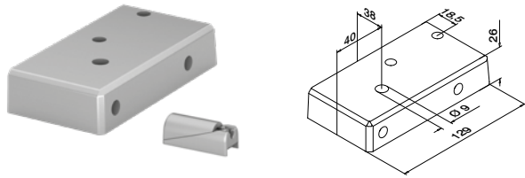
Links Inklusive Nivellierblock
